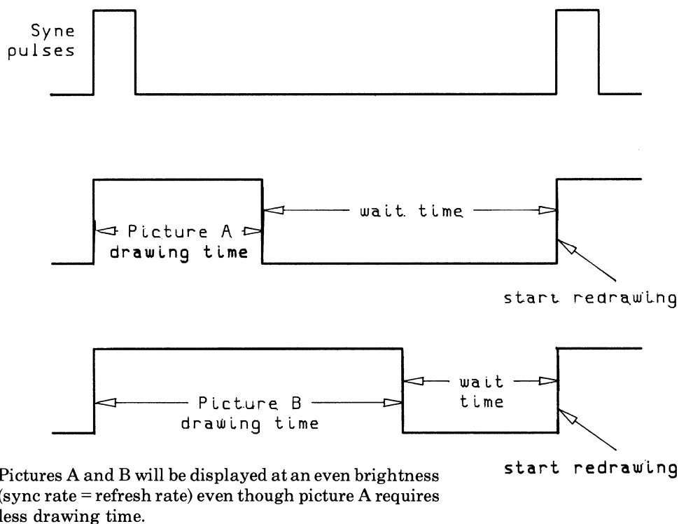
Figure 3-29. Synchronous Refresh Example
