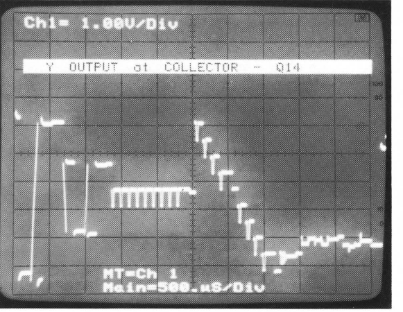
Y OUTPUT AT A1 COLLECTOR OF Q14 (TO VERTICAL CRT DEFLECTION PLATES)
