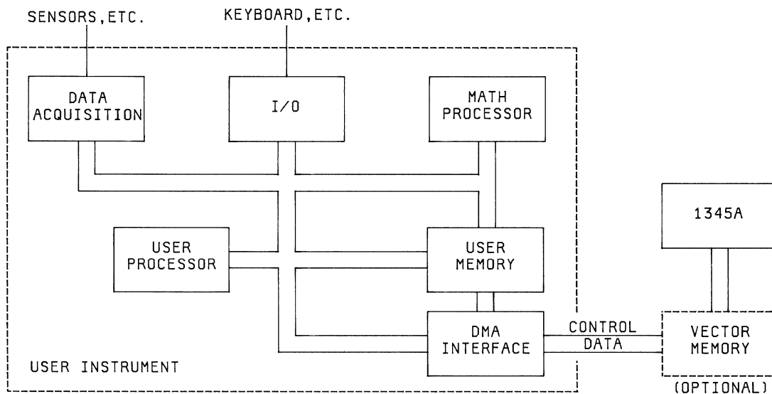
Figure 3-24. DMA Interface
