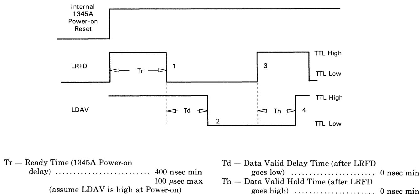
Figure 3-4. LRFD and LDAH (Ready for Data, Data Valid) Handshake
