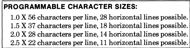
Figure 3-16. 1345A Character Display Capabilities
