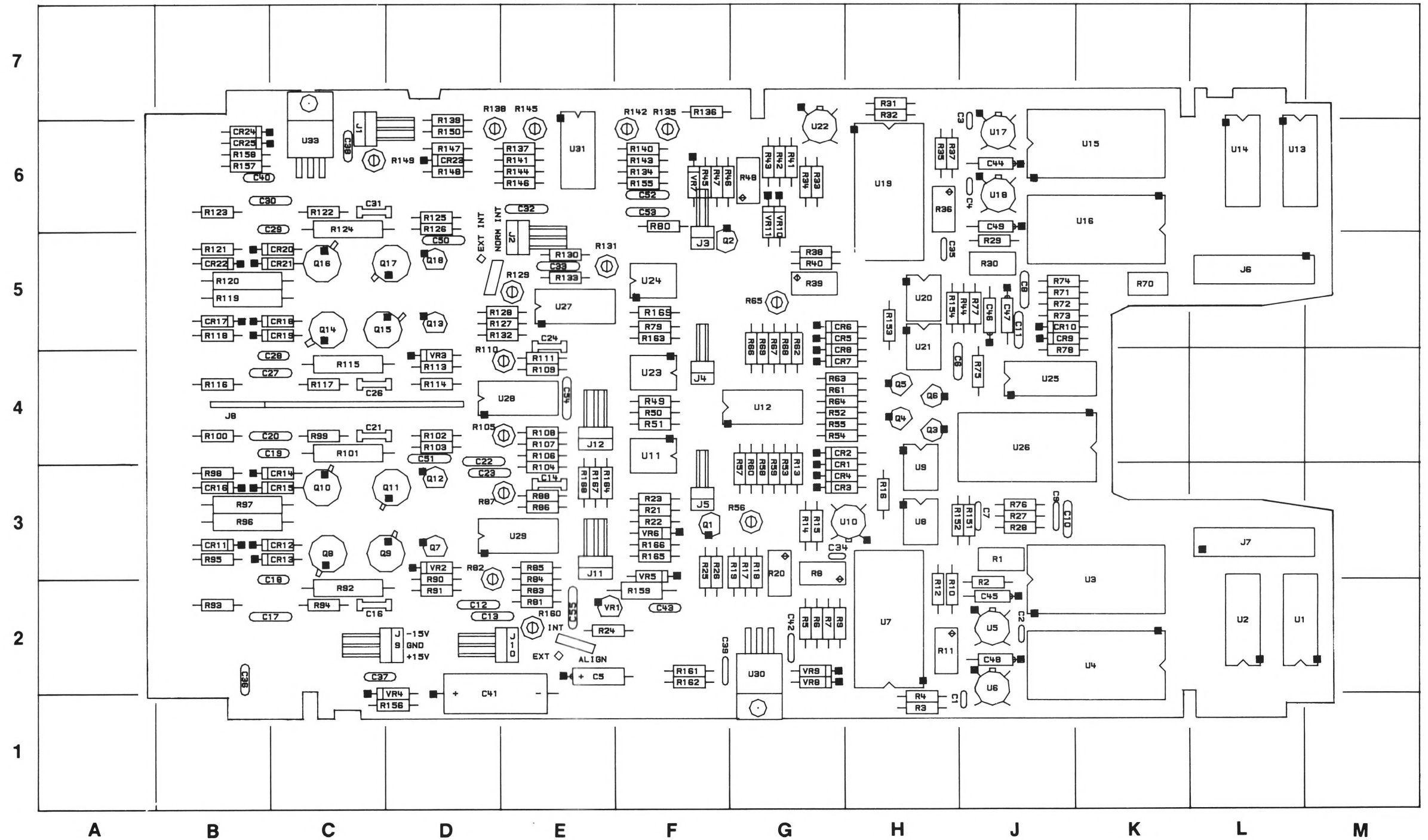
P/O Service Sheet 3A, X-Y-Z Amp/Stroke Generator (A1)
