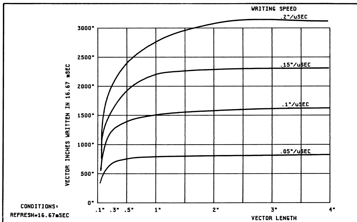
Figure 3-31. Vector Length vs Writing Speed for 60 Hz Refresh Rate
