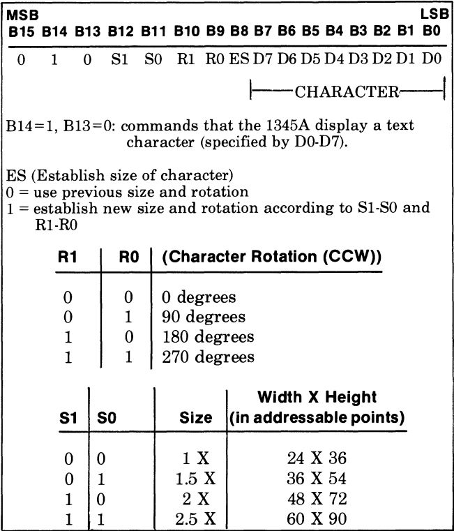
Figure 3-15. Text Command Bit Pattern
