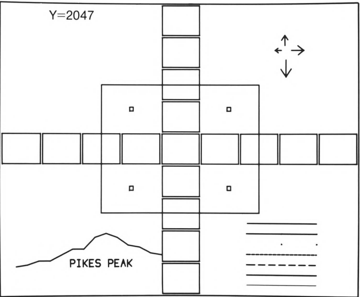
Figure 5-4. Primary Test Pattern Adjustment
