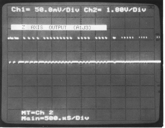
Z AUX OUTPUT AT A1J3
