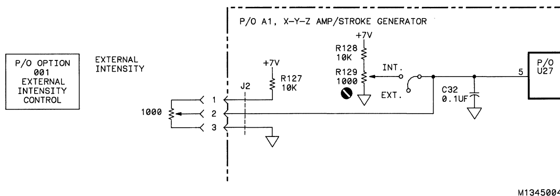
Figure 1-5. External Intensity Potentiometer Connection.
