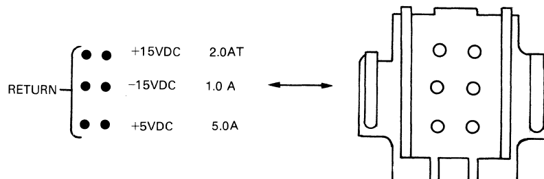
Figure 2-1. Power Connection for 1345A
