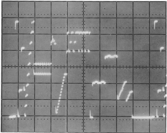
X DAC OUTPUT .05 V/DIV, 2 ms/DIV
