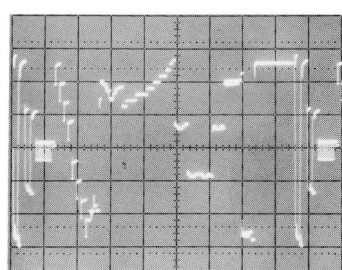
Y OUTPUT AT A1Q14 COLLECTOR (TO VERTICAL CRT DEFLECTION PLATES) 10 V/DIV, 2 ms/DIV
