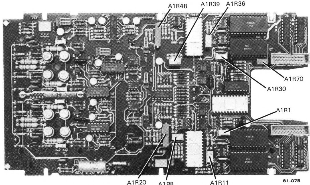
Figure 5-8. Stroke Generator and Stroke Length Adjustment Locations
