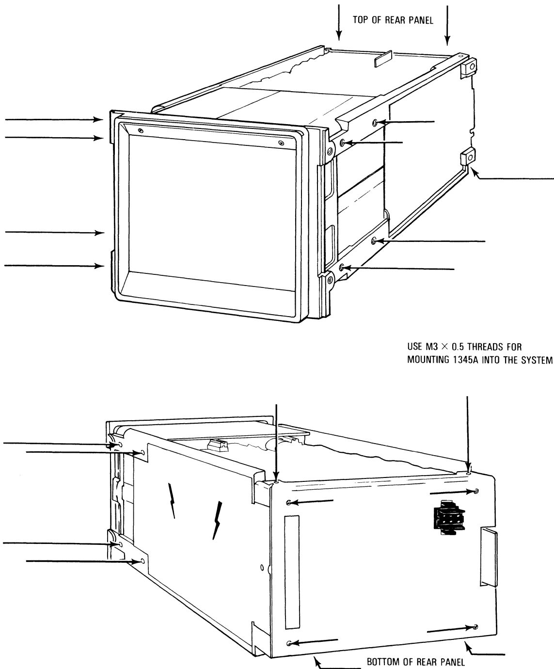
Figure 2-5. Recommended Mounting Configuration
