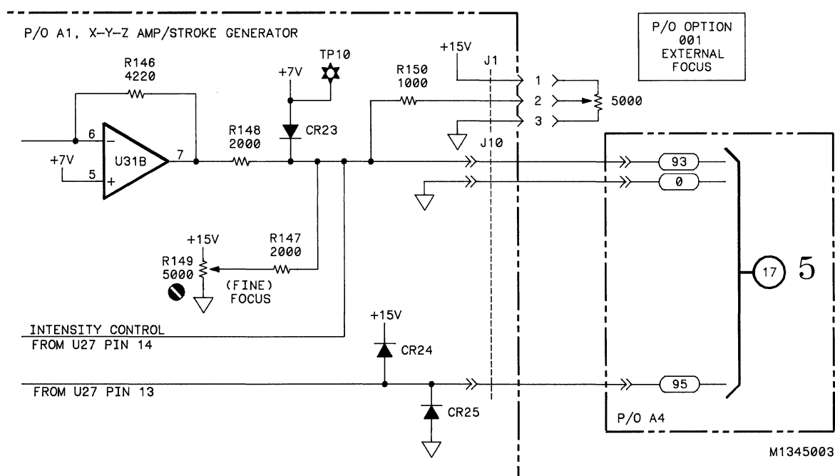
Figure 1-4. External Focus Potentiometer Connection.
