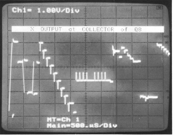
X OUTPUT AT A1 COLLECTOR OF Q8 (TO HORIZONTAL CRT DEFLECTION PLATES)
