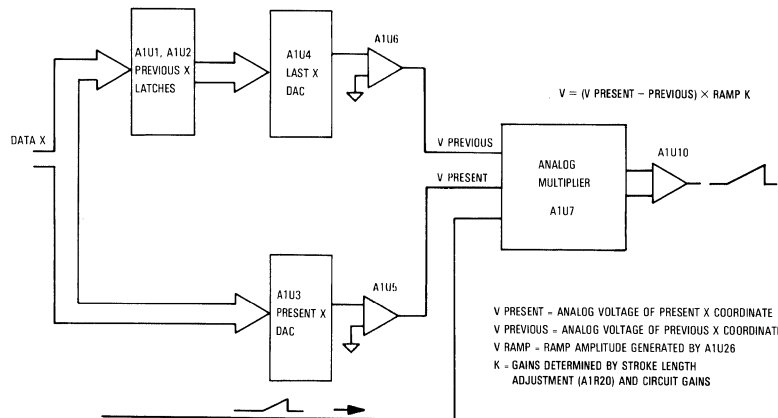
Figure 8-3. Simplified Block Diagram For Analog Multiplier
