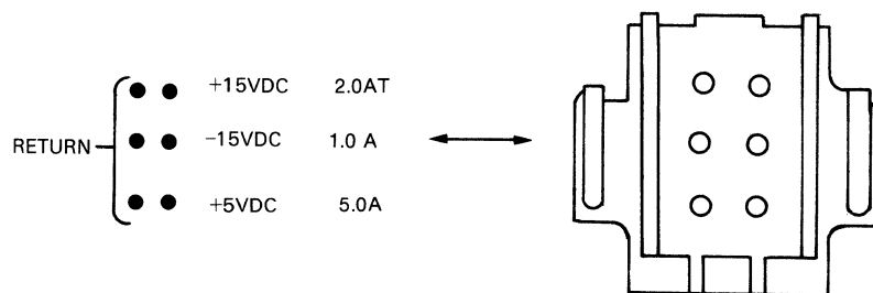
Figure 4-1. Rear Panel Power Connections
