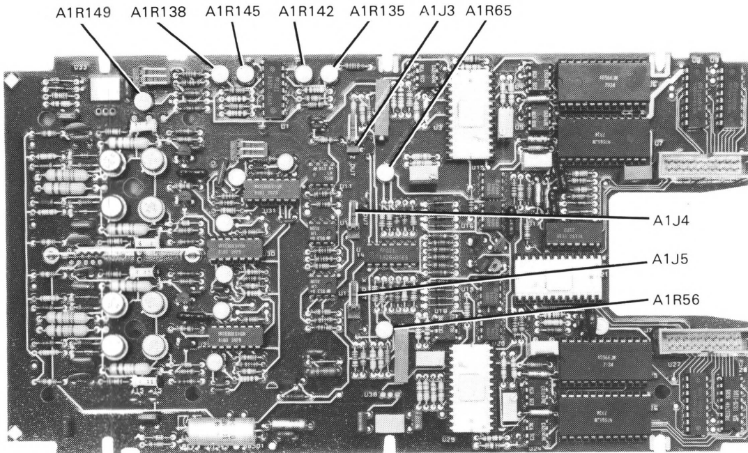
Figure 5-11. Stroke Intensity and Focus Adjustment Locations
