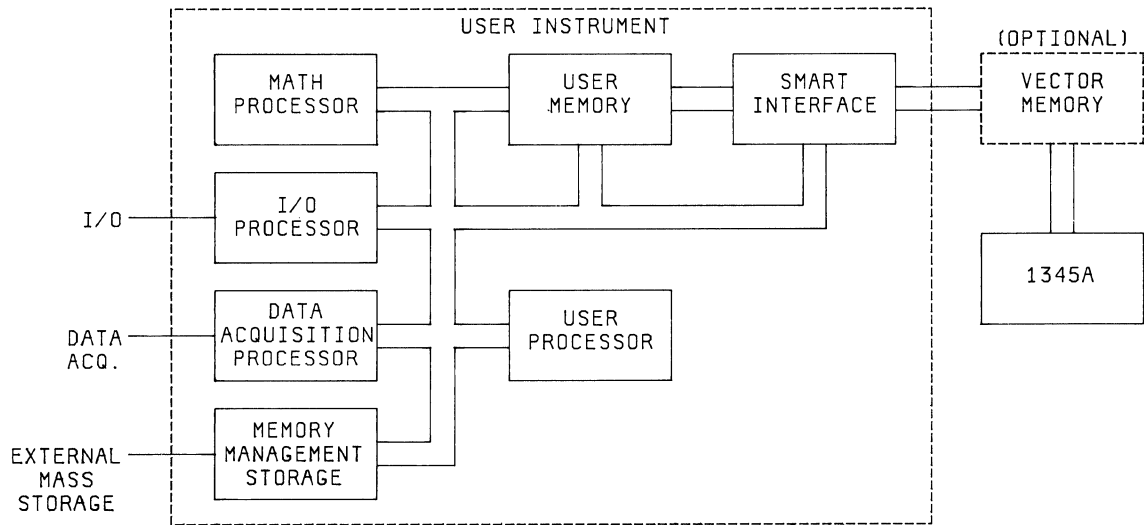
Figure 3-25. Example Smart Interface
